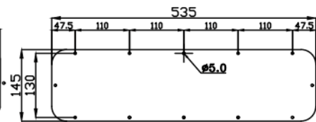
CABLE ENTRY PLATE
