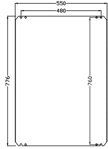
MOUNTING PLATE
