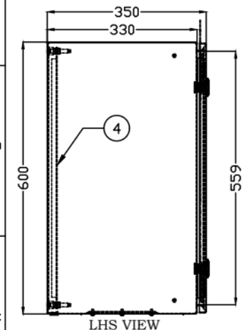
LHS VIEW
