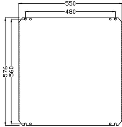
MOUNTING PLATE
