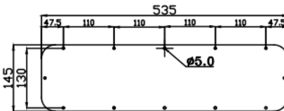
CABLE ENTRY PLATE
