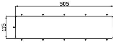
CABLE ENTRY CUTOUT
