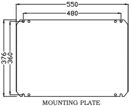
MOUNTING PLATE
