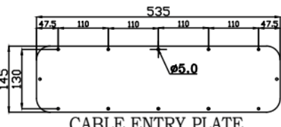
CABLE ENTRY PLATE
