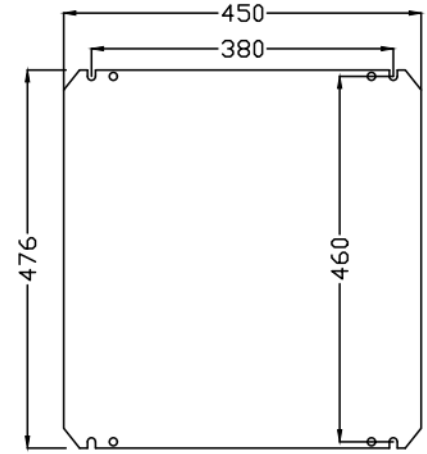
MOUNTING PLATE
