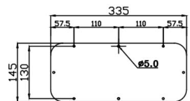
CABLE ENTRY PLATE
