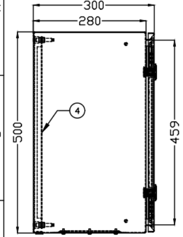
LHS VIEW
