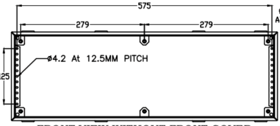
FRONT VIEW WITHOUT FRONT COVER
