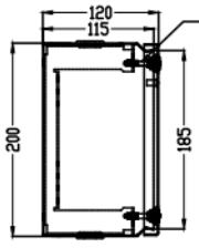
LHS VIEW
