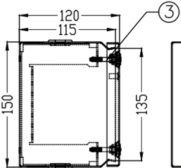
LHS VIEW
