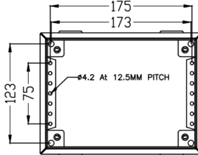
FRONT VIEW WITHOUT FRONT COVER
