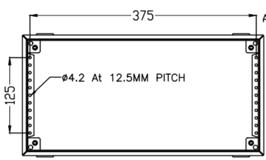
FRONT VIEW WITHOUT FRONT COVER
