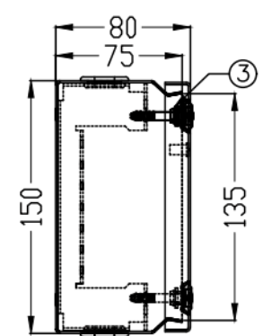
LHS VIEW
