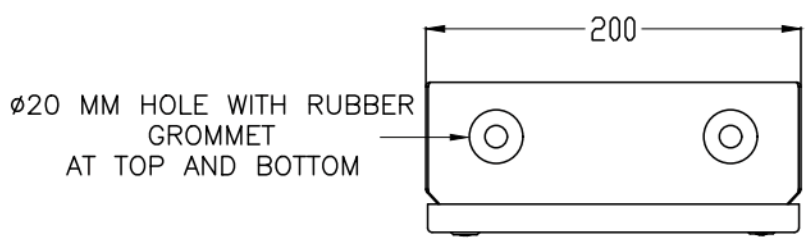
TOP VIEW
