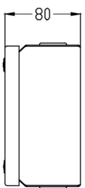
RHS VIEW
